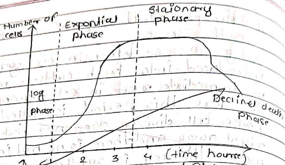
Fig. sigmoid curve for bacterial growth. Shows different phases of growth.
