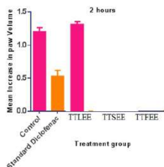
Figure no. 4 Effect of compounds on mean increase in paw volume after 2 hour on drug. The data were expressed as mean ± SEM.
